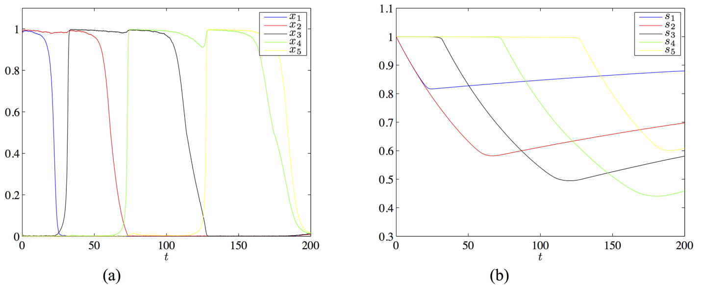
Fig 3. The chain of four patterns in the network of 5 neurons with the transition matrix Eq (25) and the parameters I = 0.3 , \lambda = 3.4 , \mu = 3.1 , \tau_r = 400 and U = 0.01 . Panel (a) shows the evolution of the firing rate variables, panel (b) shows the evolutions of the synaptic variables.
